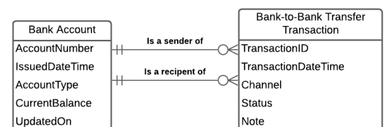
Crow's Foot Notation
